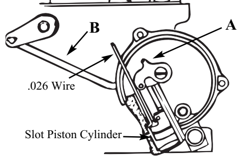
Choke piston linkage Figure 10
