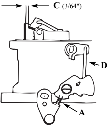
Fast idle linkage Figure 11
